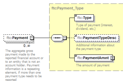
Figure 13 - Payment element
