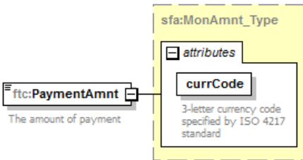
Figure 14 - PaymentAmt element
