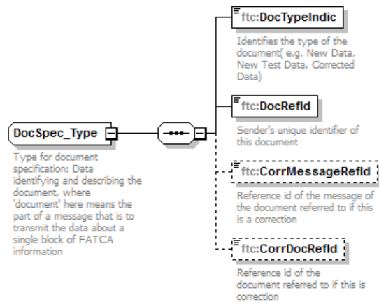
Figure 3 - DocSpec_Type
