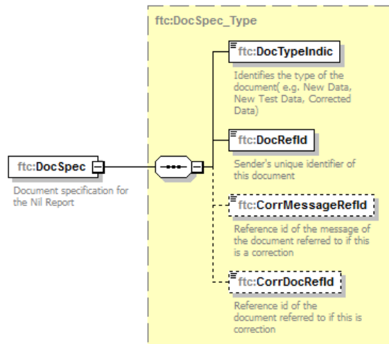
Figure 18 - DocSpec element
