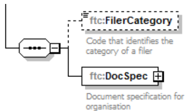
Figure 8 - FilerCategory
