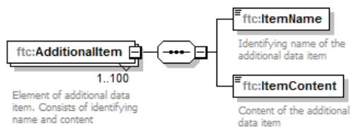
Figure 16 – AdditionalItem element
