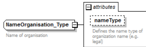
Figure 7 - NameOrganisation_Type
